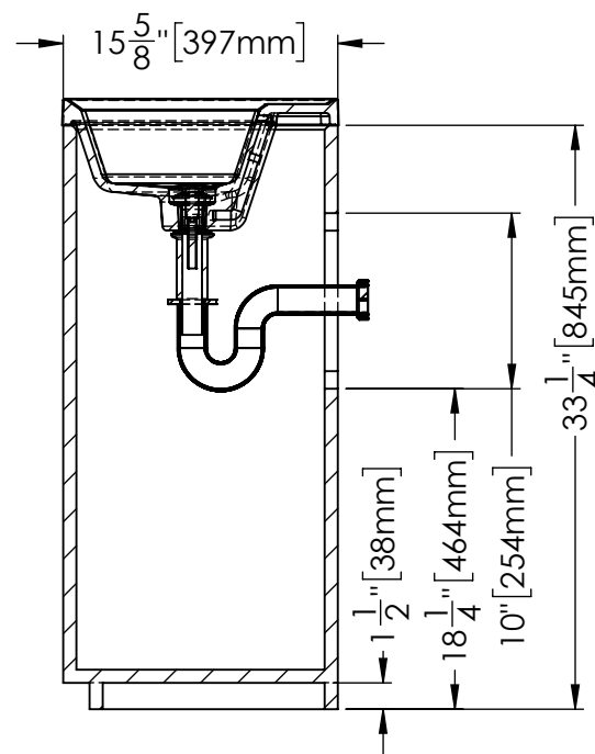
SECTION C-C
