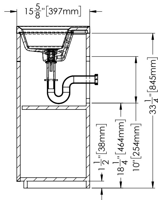
SECTION F-F
