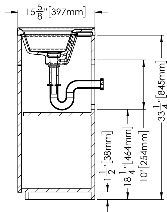
SECTION E-E
