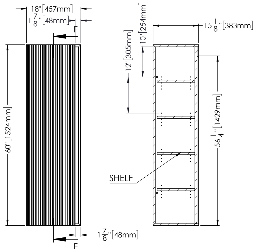
SECTION F-F SCALE 1 : 16
