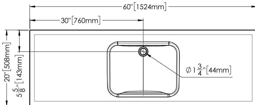
Top View
